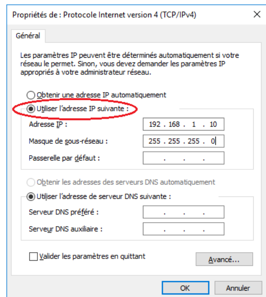
Illustration 27: modifier l'IP
